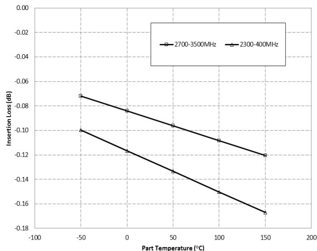
XMC0204E2-03G Typical Insertion Loss Derating Curve
