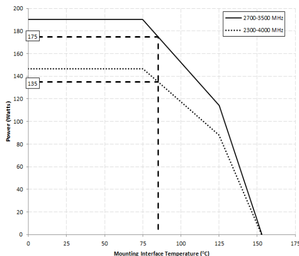
XMC0204E2-03G Power Derating Curve
